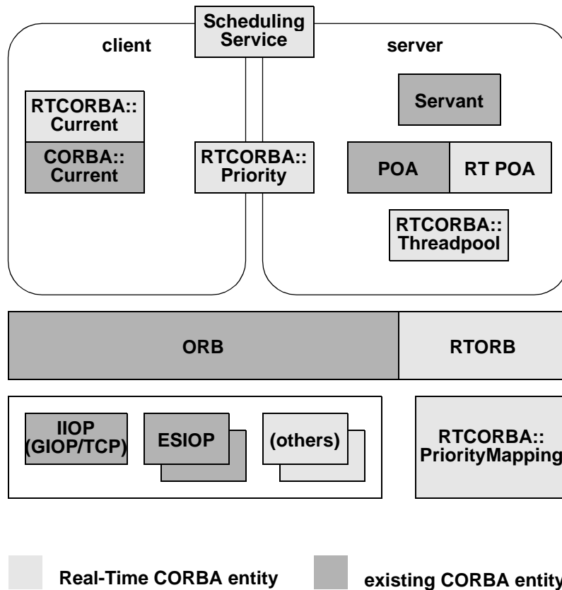
Figure 1-1 Real-Time CORBA Extensions
